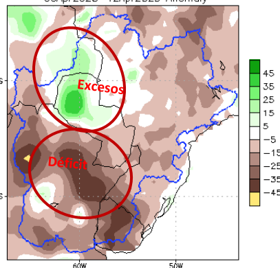
NCEP GFS Ensemble Forecast 8-14 Day Precipitation (mm) from: 30Mar2025 for La_Plata_Basin 06Apr2025-12Apr2025 Anomaly
