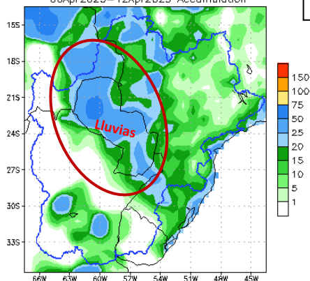
NCEP GFS Ensemble Forecast 8-14 Day Precipitation (mm) from: 30Mar2025 for La_Plata_Basin 06Apr2025-12Apr2025 Accumulation
